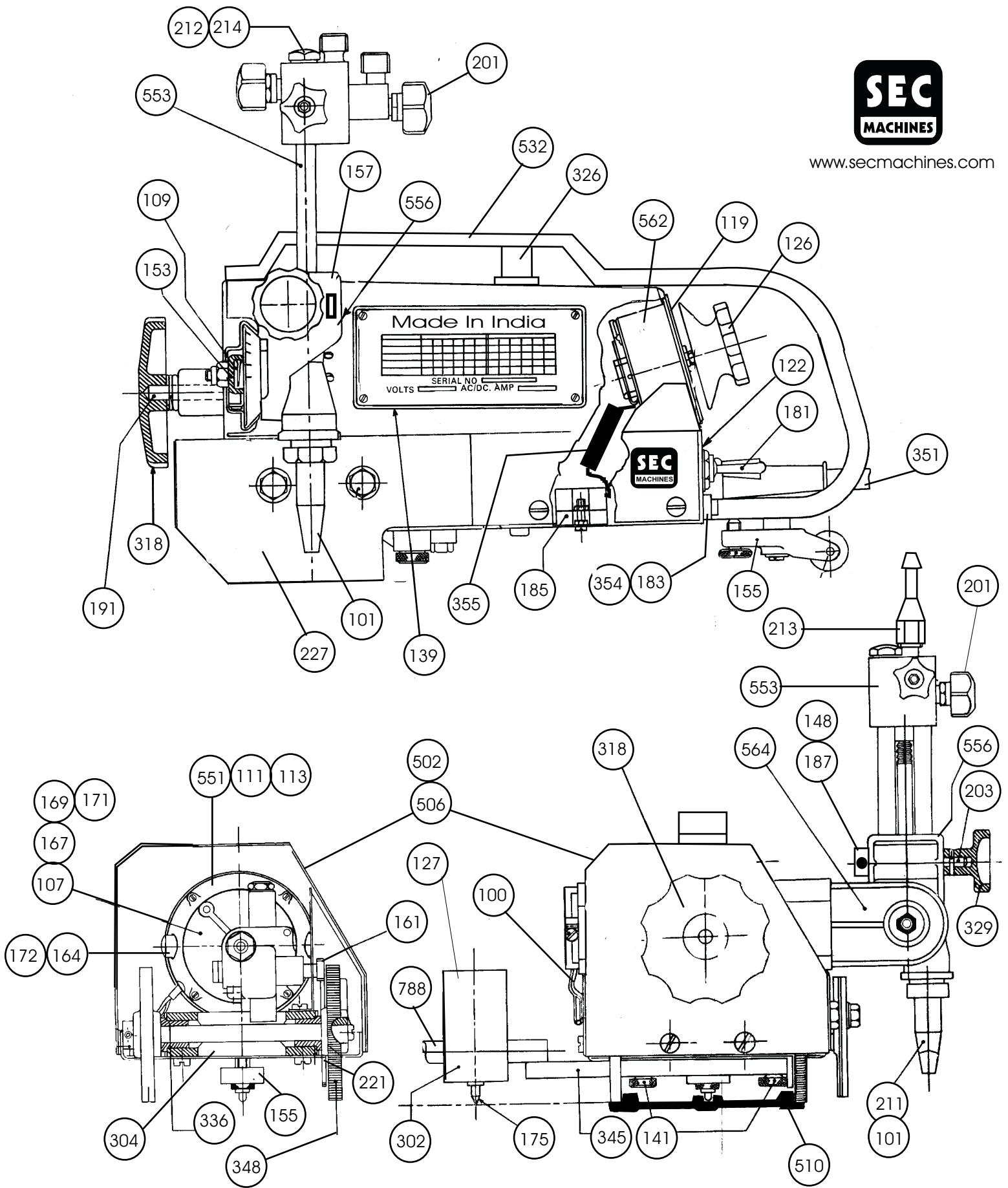
Oxy 200 Spares' General Arrangement Drawing
